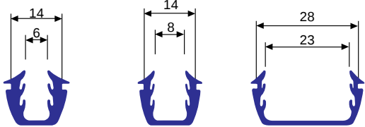
MONOLITICO 6 mm. MONOLITICO 8 mm. TERMOPANEL 23 mm.
